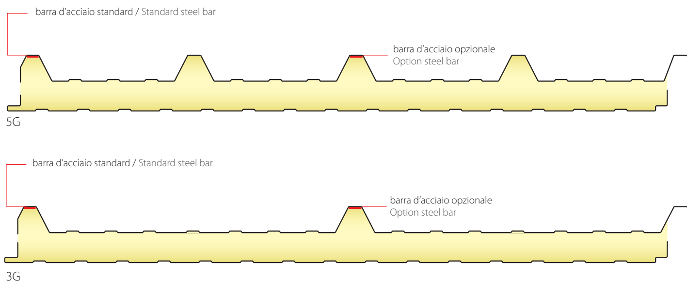
Profile types
